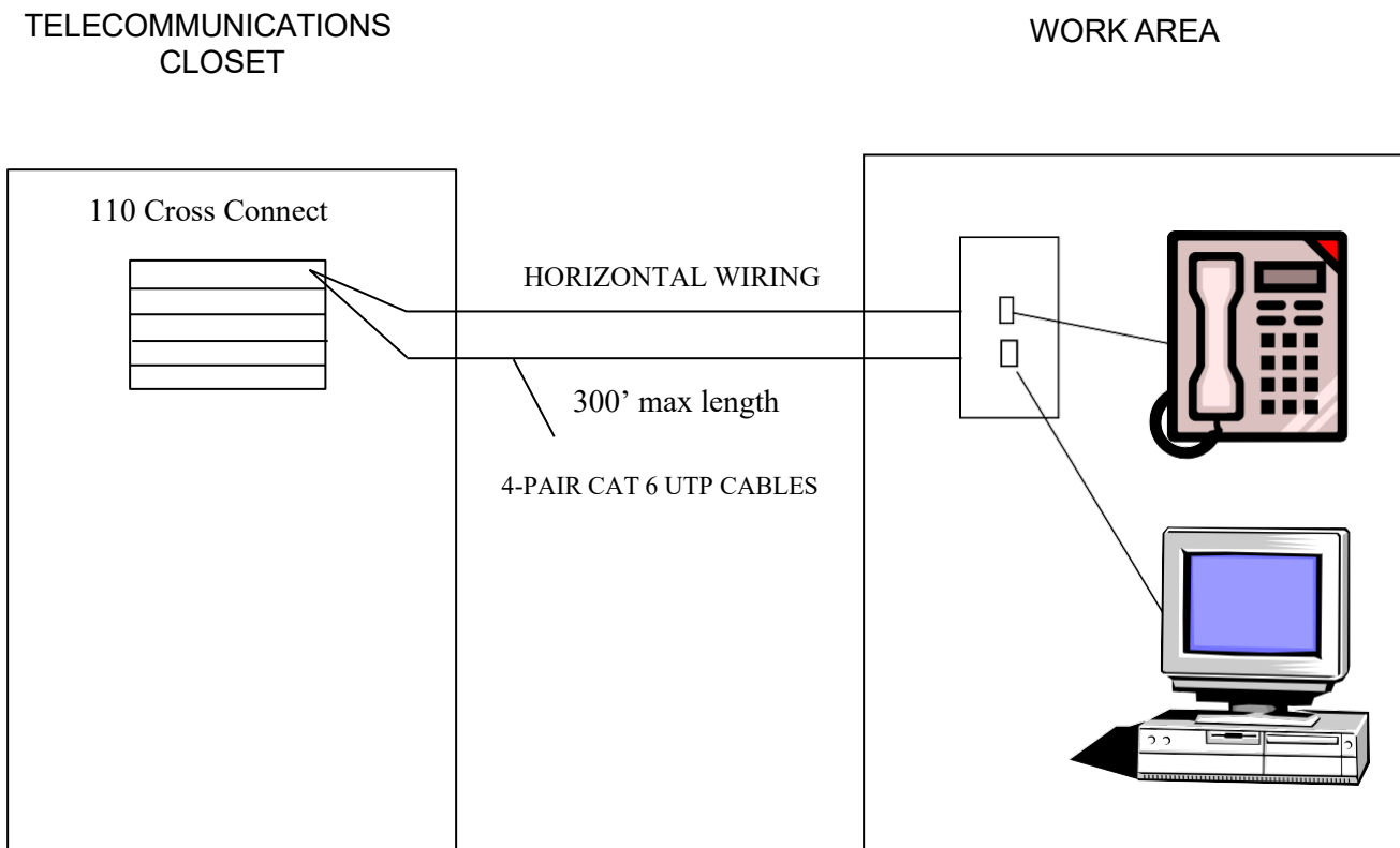
FIGURE 1.1 Typical Horizontal and Work Area Wiring
