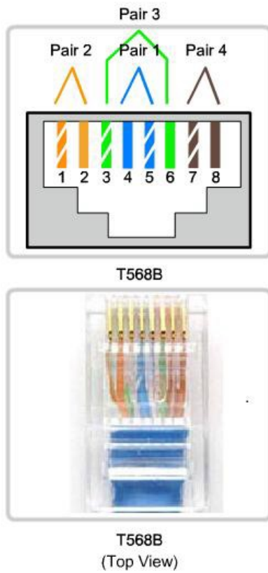
FIGURE 1.2: Eight-Position Jack Pin/Pair Assignments (Designation T568B)
